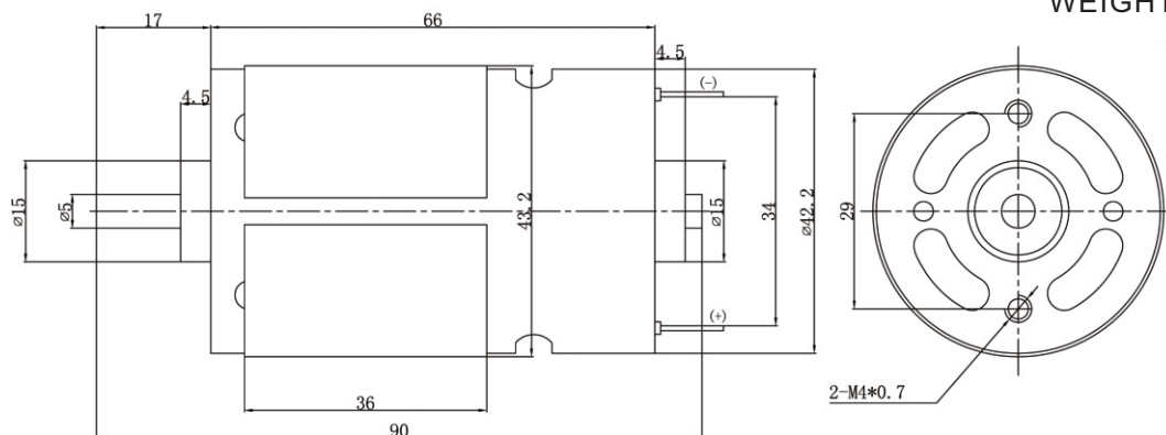
DRAWING (MM)
