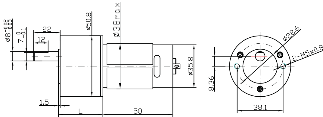
DRAWING (MM)
