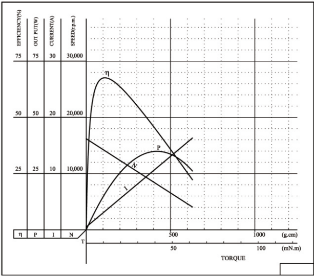
MODEL: DSD-380SH-4045
