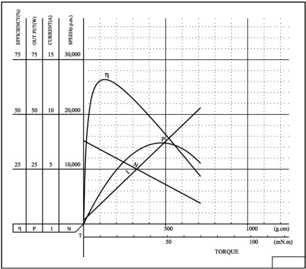
MODEL: DSD-380SH-3270
