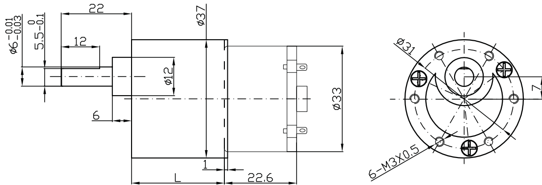
DRAWING (MM)
